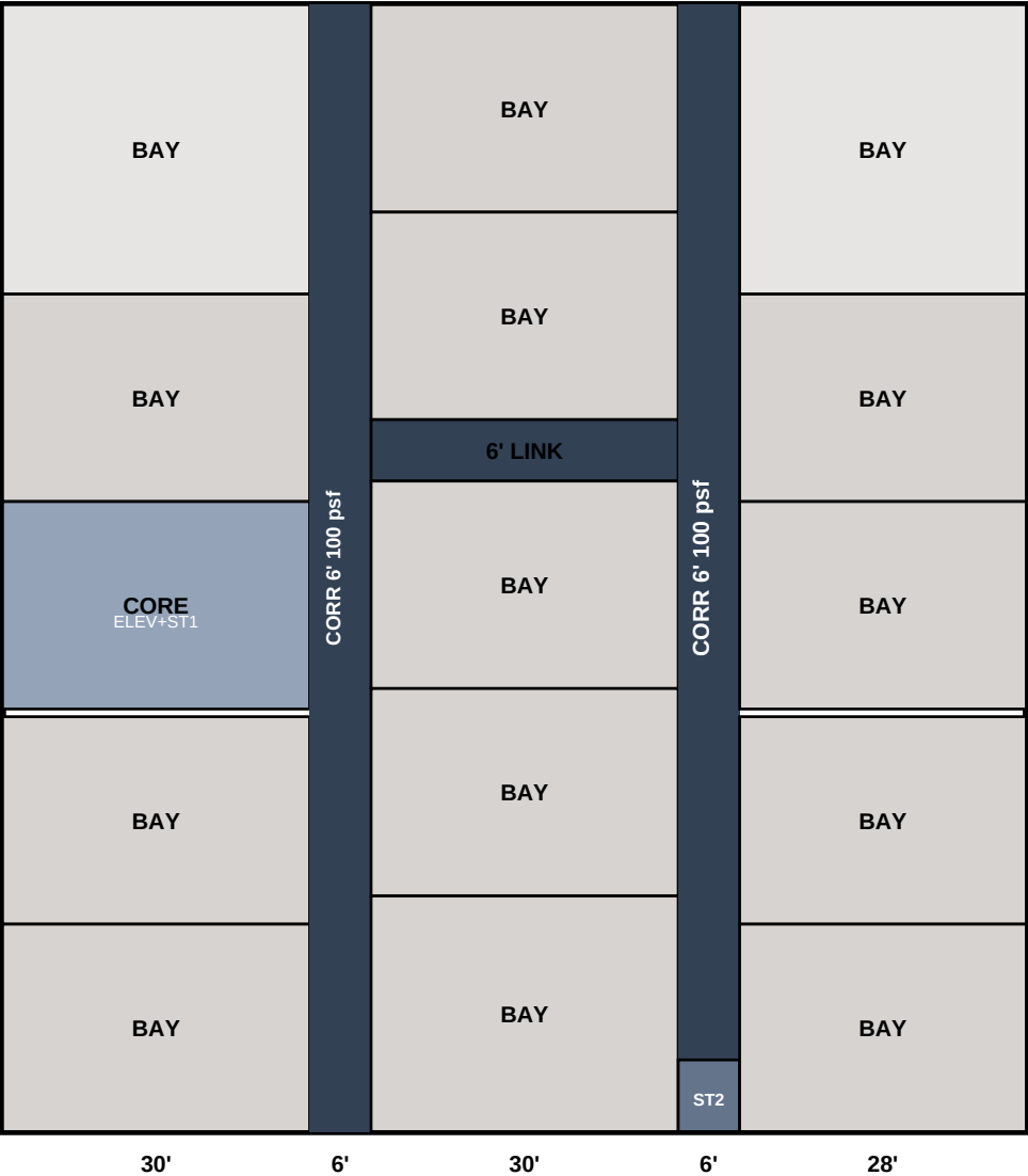
INTERIOR PACK (TI) — STEEL USES COLUMN GRID ON S-1
